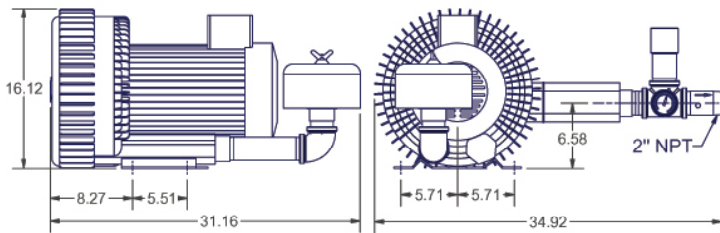
KPHRB1002 - Pressure Kit Drawing
