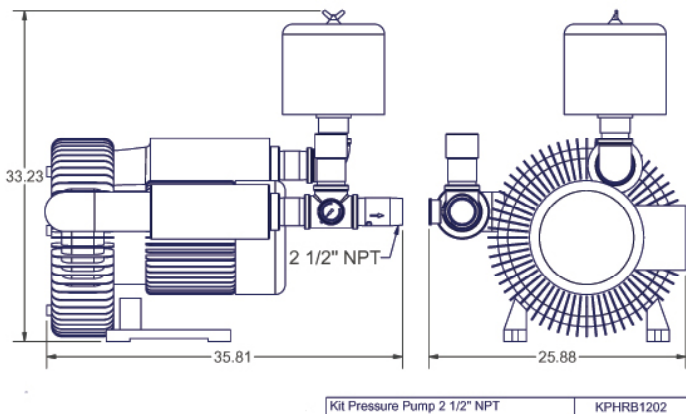
KPHRB1202 - Pressure Kit Drawing
