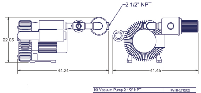
KVHRB1202 - Vacuum Kit Drawing
