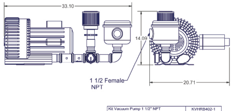
KVHRB402S/1 - Vacuum Kit Drawing
