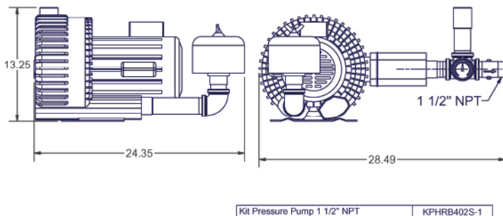
KPHRB402S/1 - Pressure Kit Drawing
