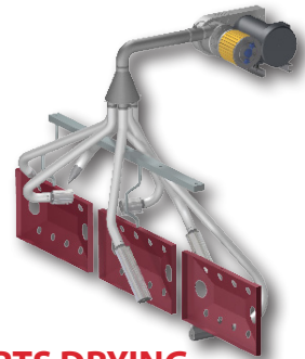
PARTS DRYING
