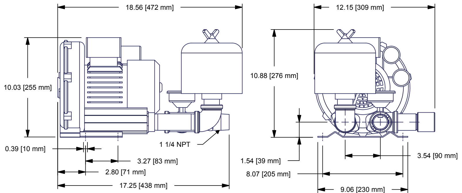
KPHRB101 - Pressure Kit Drawing
