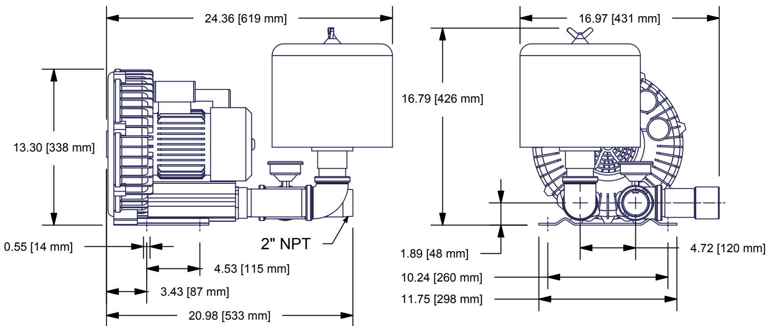
KPHRB301- Pressure Kit Drawing
